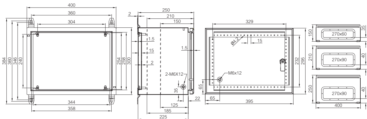
CAB SL 300x400x150-250 mm
