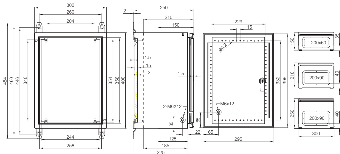
CAB SL 400x300x150-250 mm
