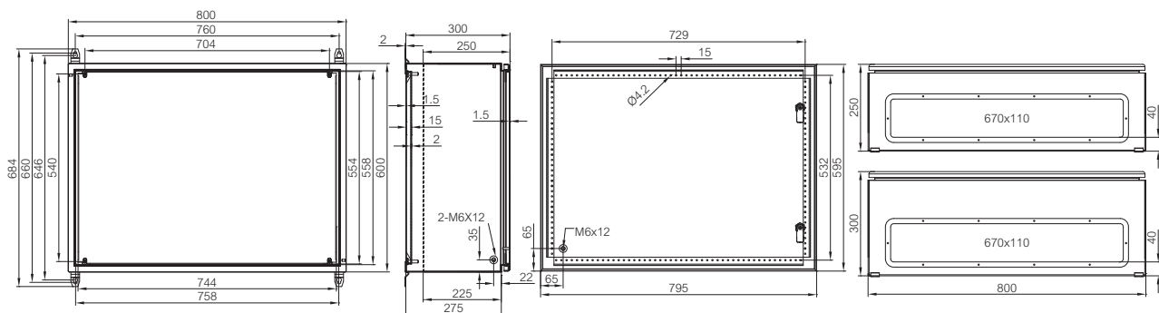
CAB SL 600x800x250-300 mm
