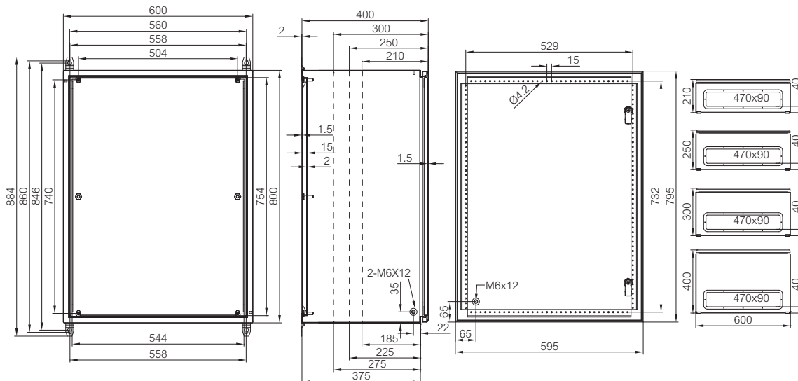
CAB SL 800x600x210-400 mm
